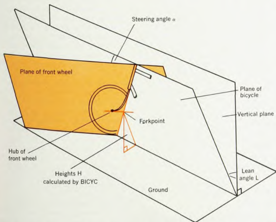
A TRICKY TRIGONOMETRICAL PROBLEM. We need to know H , the height of the forkpoint from the ground, for a leaning bicycle. Subroutine BICYC calculates both the vertical height and the height in the plane of the bike. —FIG. 3
