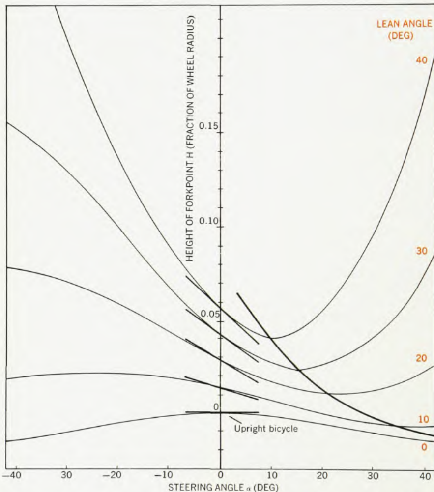
COMPUTERIZED BICYCLES. These data, from BICYC output, show that the minimal height of the forkpoint occurs nearer to the straight-ahead position for greater angles of lean. Note also that dH/d\alpha varies linearly with lean angle L for small L . Curves, computed for typical steering geometry (20-deg fork angle, 0.2 radii front projection), are vertically staggered for clarity. —FIG. 4
