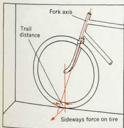
SIDWAYS FORCE on front tire produces a torque about the steering axis, so tending to lower the center of gravity of the bicycle. —FIG. 6
