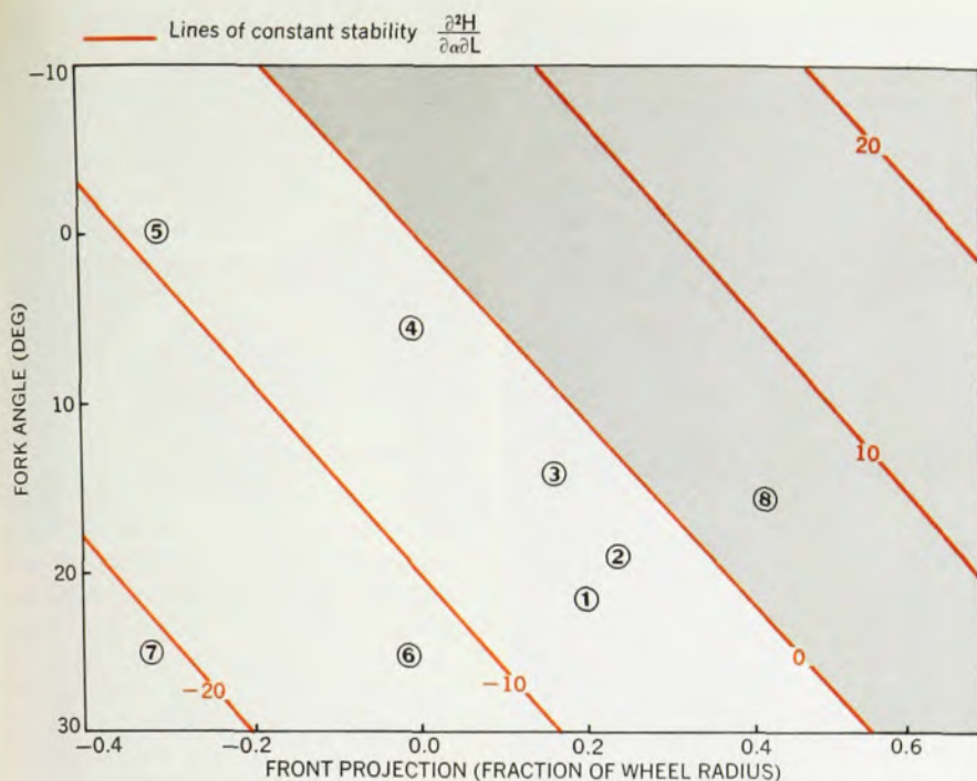
STABLE AND UNSTABLE BICYCLES. On this plot of fork angle versus front projection the \frac{d^2H}{da^2dL} lines are lines of constant stability. Grey area shows the unstable region. Point 1 is a normal modern bicycle; 2 is a racing bike. 3 and 4 are high-wheelers (or "penny-farthings") from the 1870's. Point 5 is an 1887 Rudge machine, and 6 is a Lawson "Safety" of 1879. Point 7 is URB III, and point 8, the only unstable bicycle, is of course URB IV. —FIG. 5
